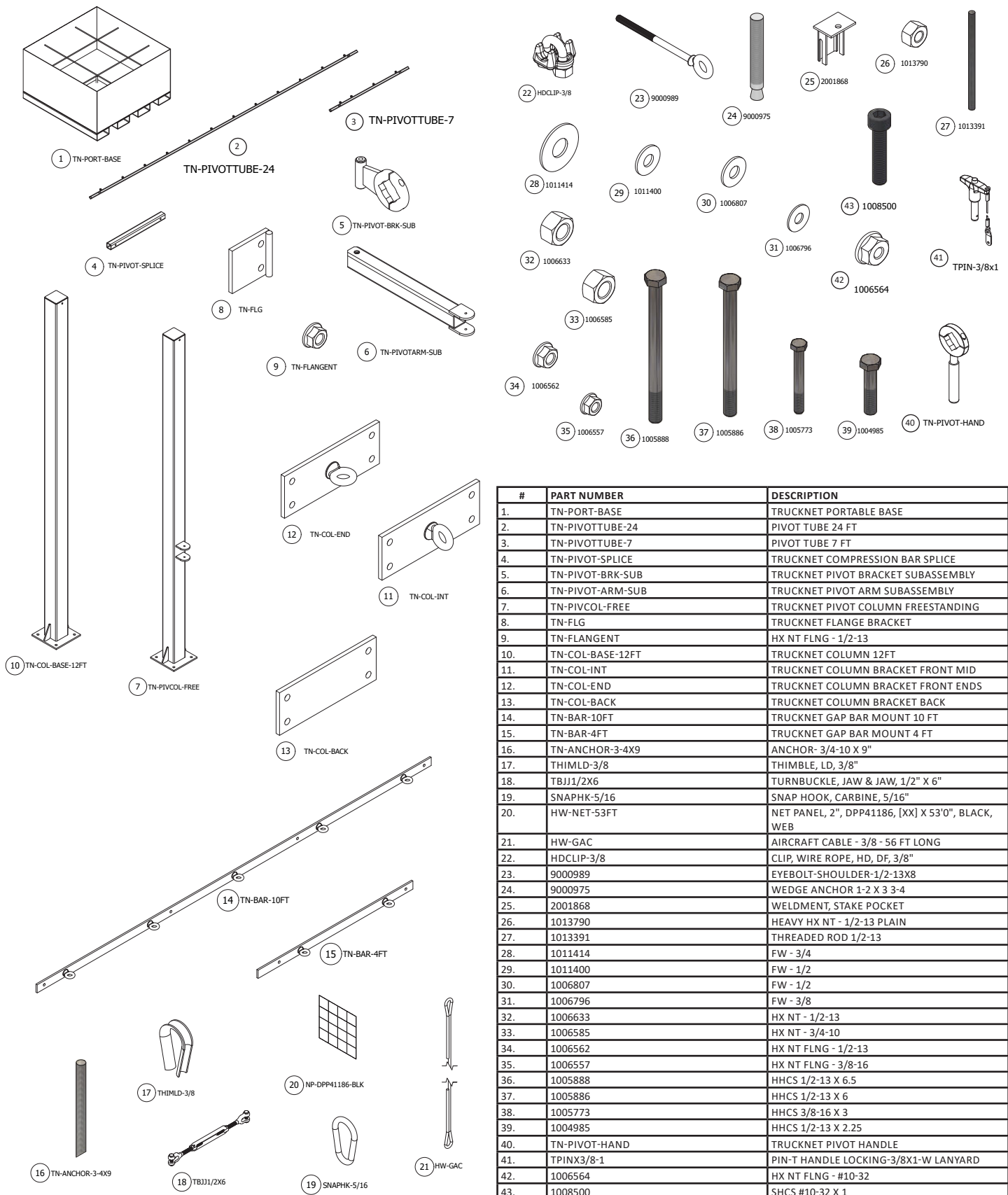
Figure 1 - Components
