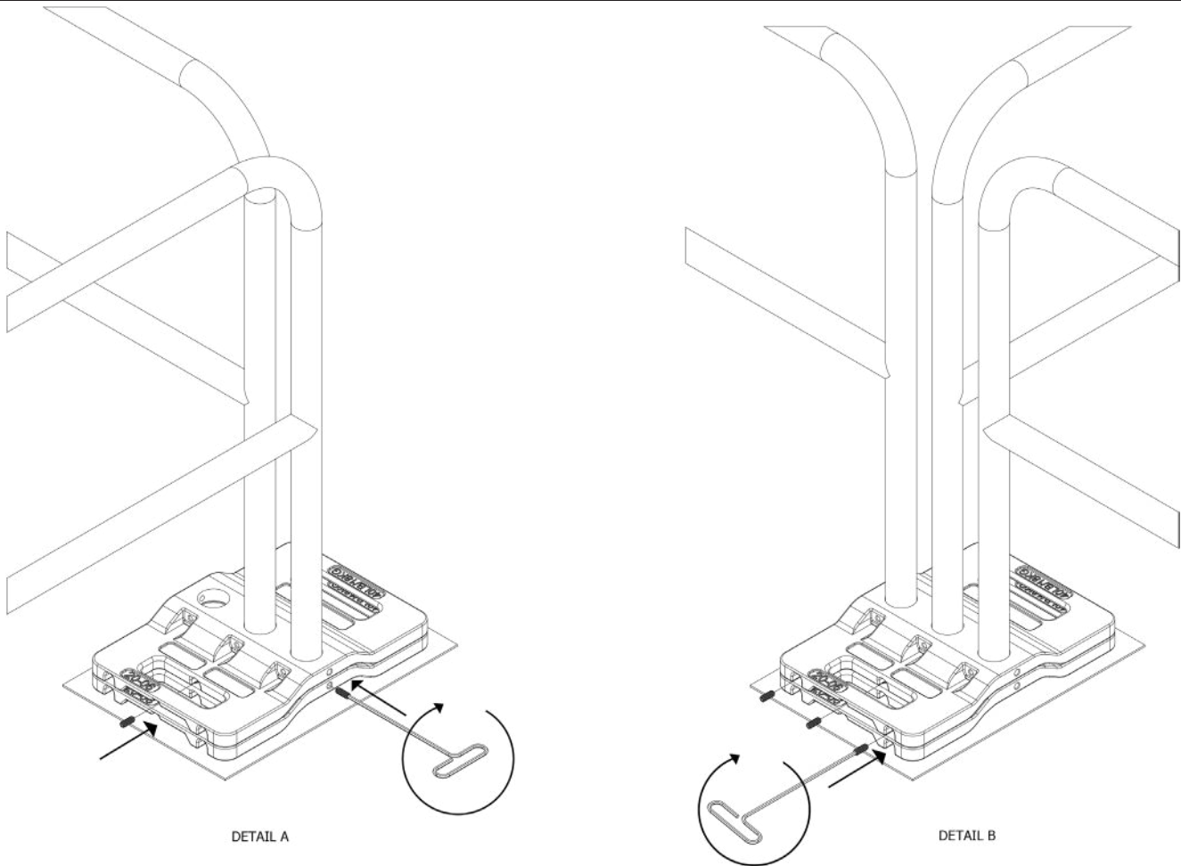
Figure 3 - Post/Base Connection
