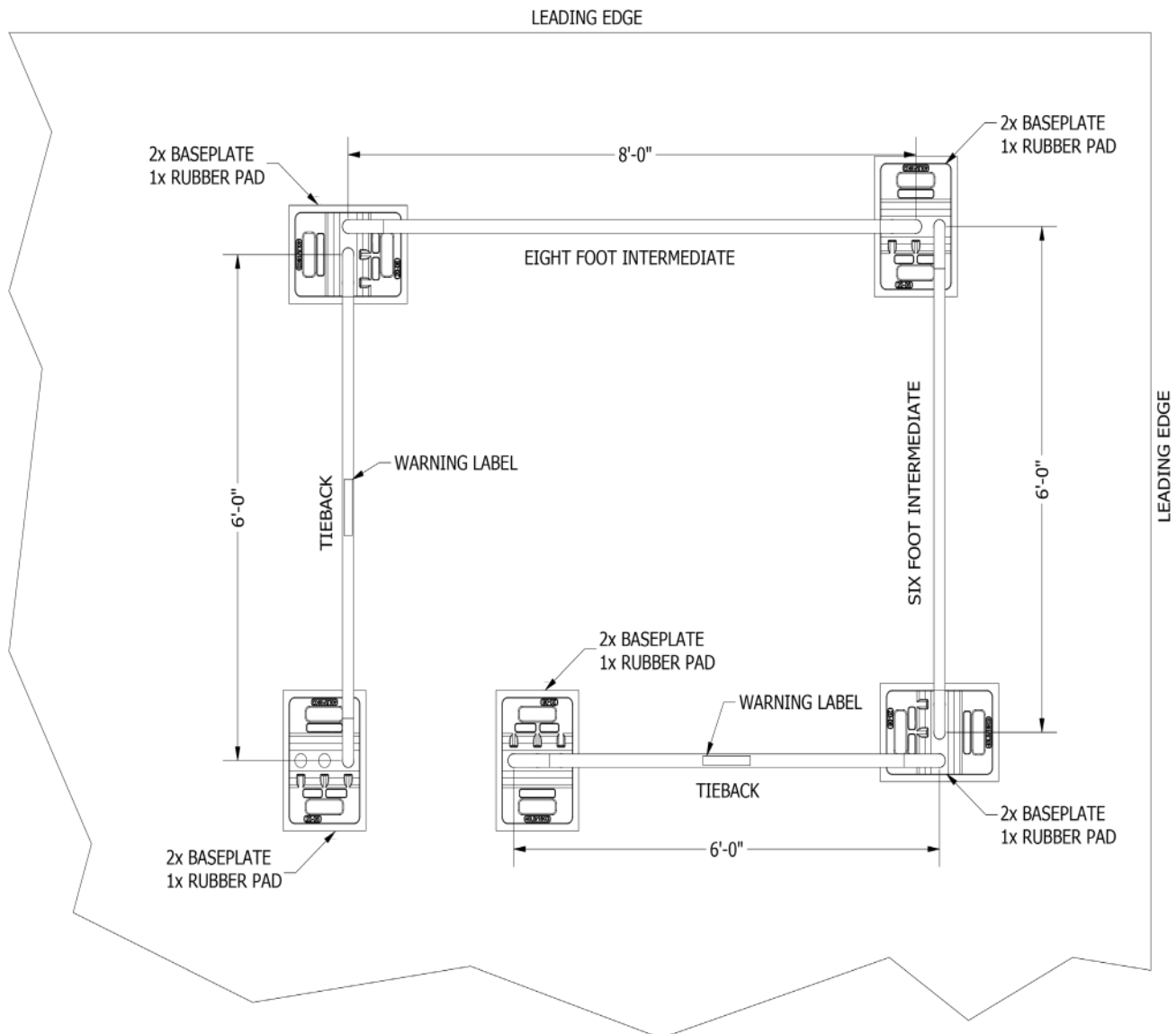
Figure 2 - Typical Layout
