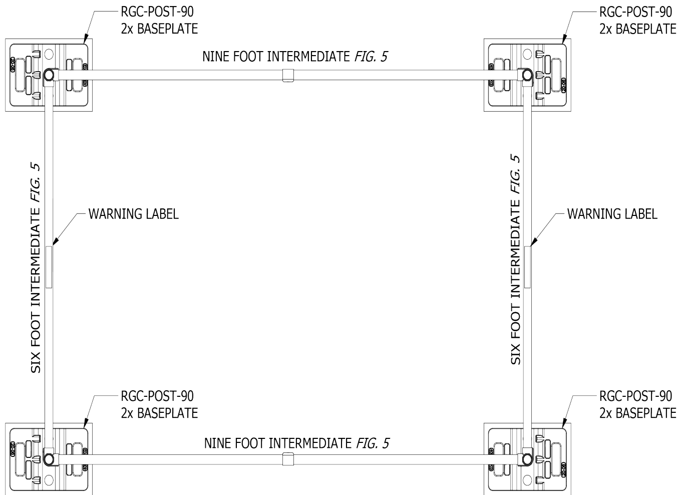
Figure 6 - Skylight Rails
