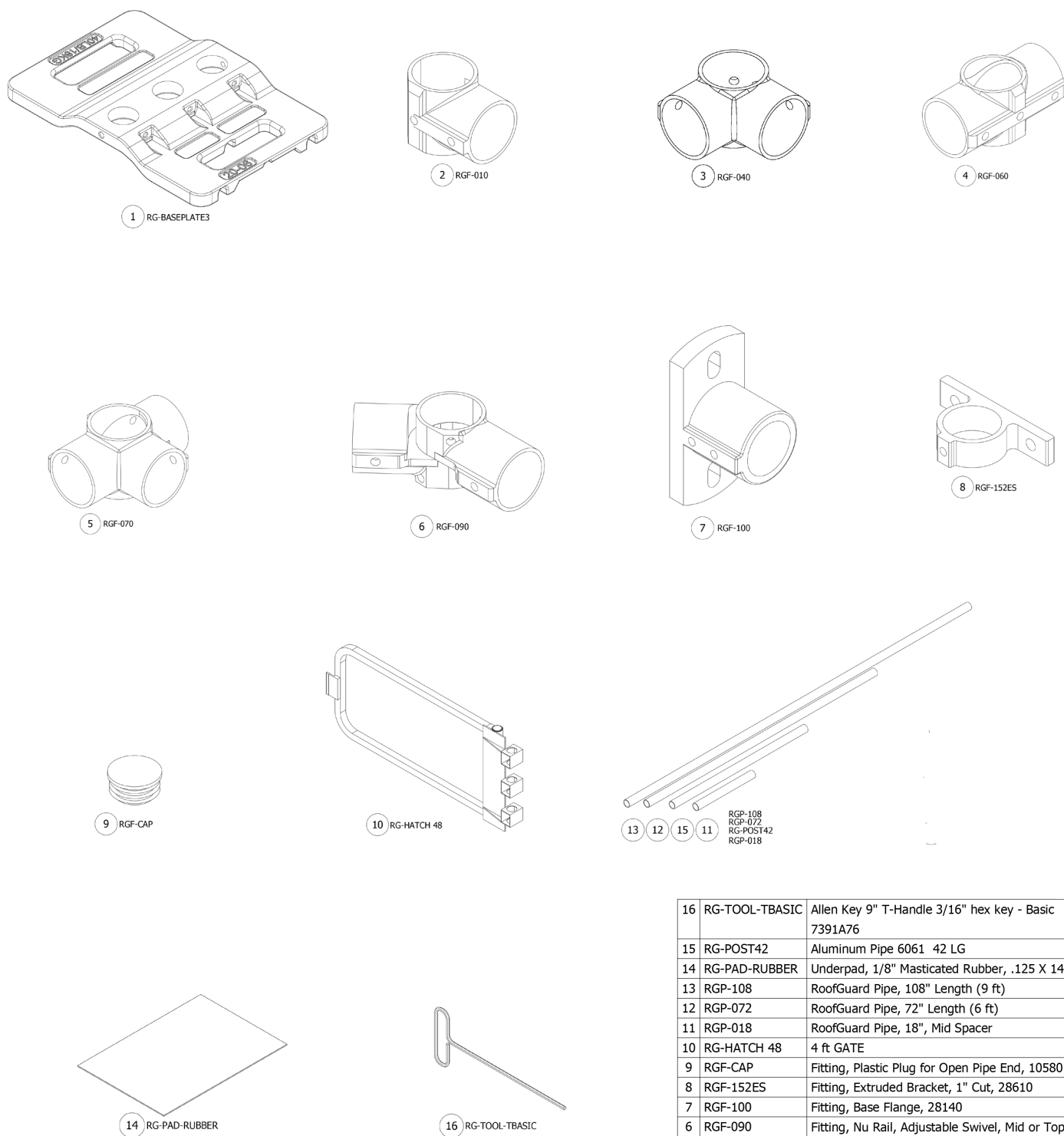
Figure 1 - Component Identification
