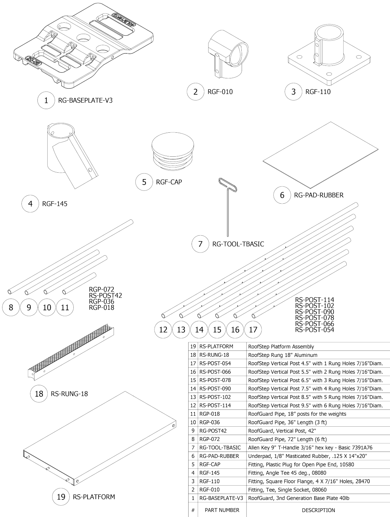
Figure 1 - Component Identification
