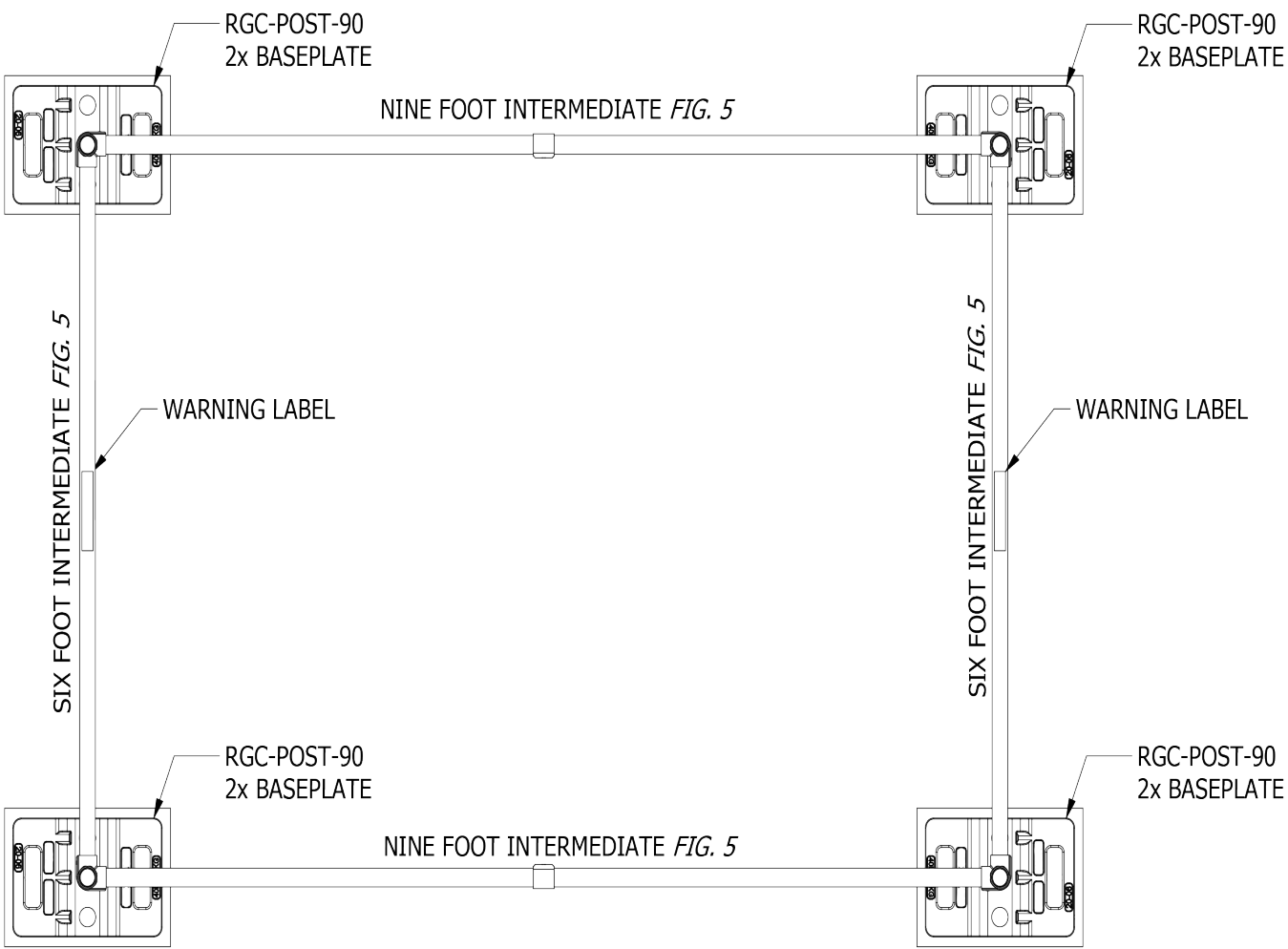
Figure 6 - Skylight Rails
