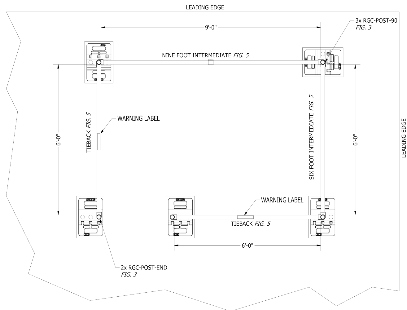
Figure 2 - Typical Layout
