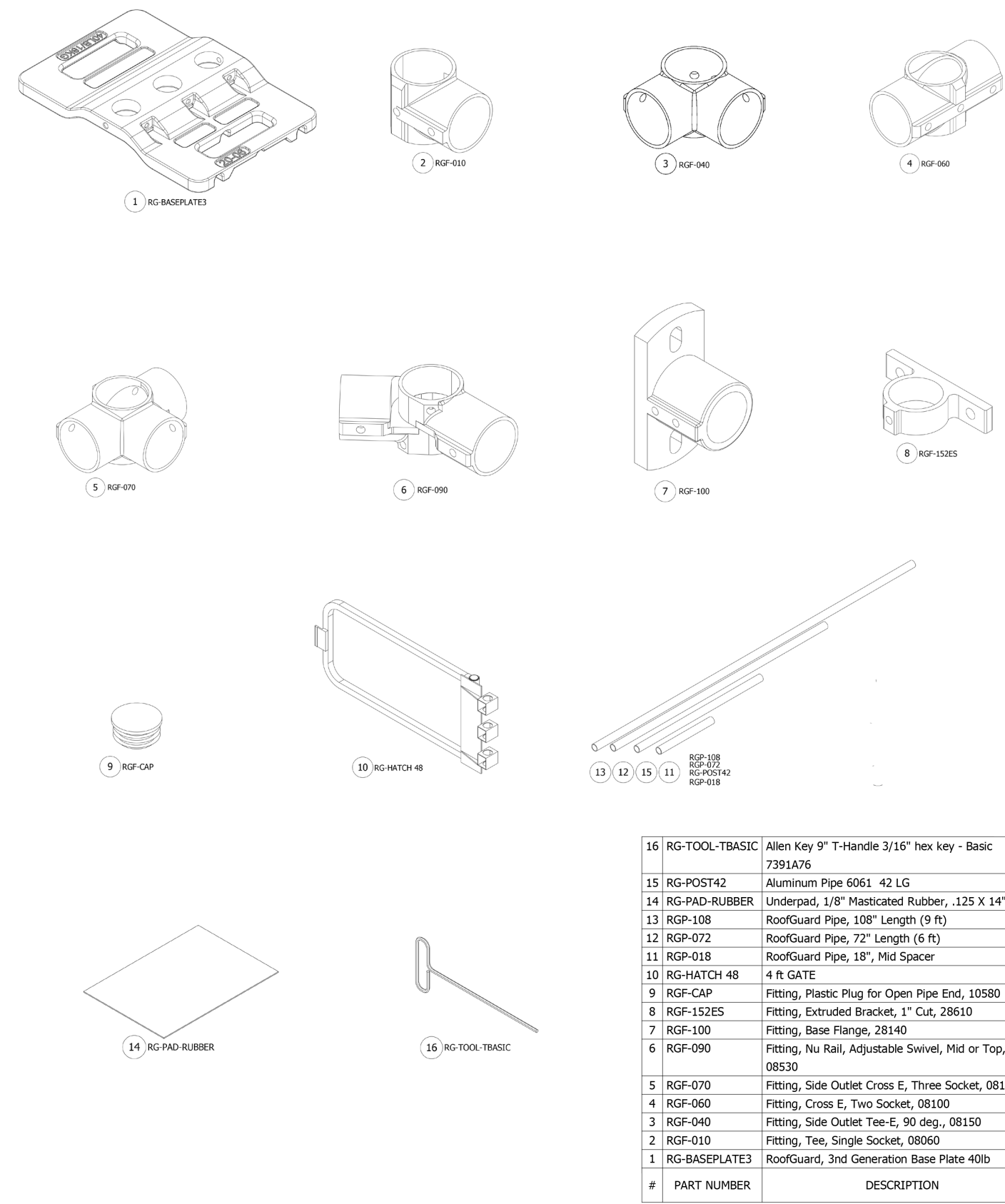
Figure 1 - Component Identification
